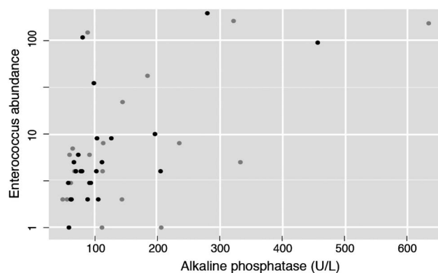
Figure 4 Positive correlation between Enterococcus abundance and alkaline phosphatase (ALP), a clinical marker for cholestasis and primary sclerosing cholangitis (PSC) progression (n=87, Spearman \rho=0.29 , adjusted p value=0.012199). Black dots correspond to patients with PSC without cirrhosis or liver transplantation. Grey dots correspond to patients with PSC with either cirrhosis or liver transplantation.
